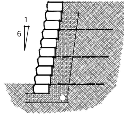
Engineered Retaining Wall
