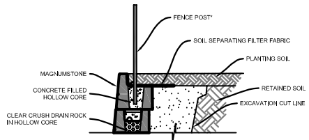
FENCE THROUGH HOLLOW CORE
