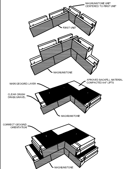
INSIDE CORNER
