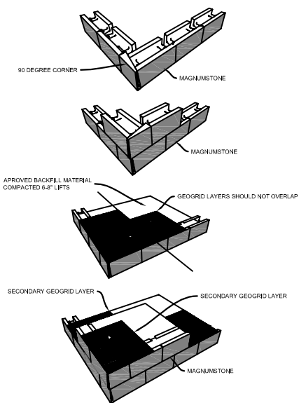
OUTSIDE CORNER
