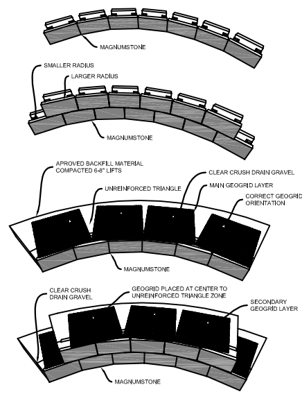
INSIDE CURVE
