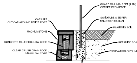
GUARD RAIL
