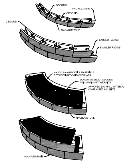
OUTSIDE CURVE
