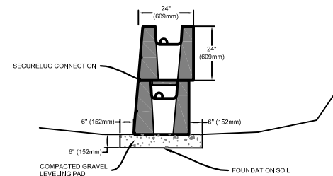
LEVELING PAD
