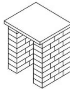
Wood Storage 38" x 32" x 28" 965.2 x 813 x 711 mm
