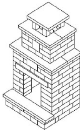
Fireplace 78" x 44" x 40" 1981 x 1118 x 1016 mm
